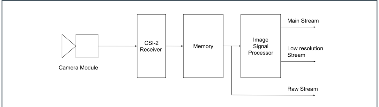
Figure 8: Camera Pipeline
