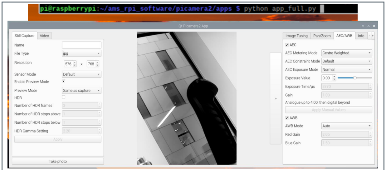
Figure 11: App_full.py
