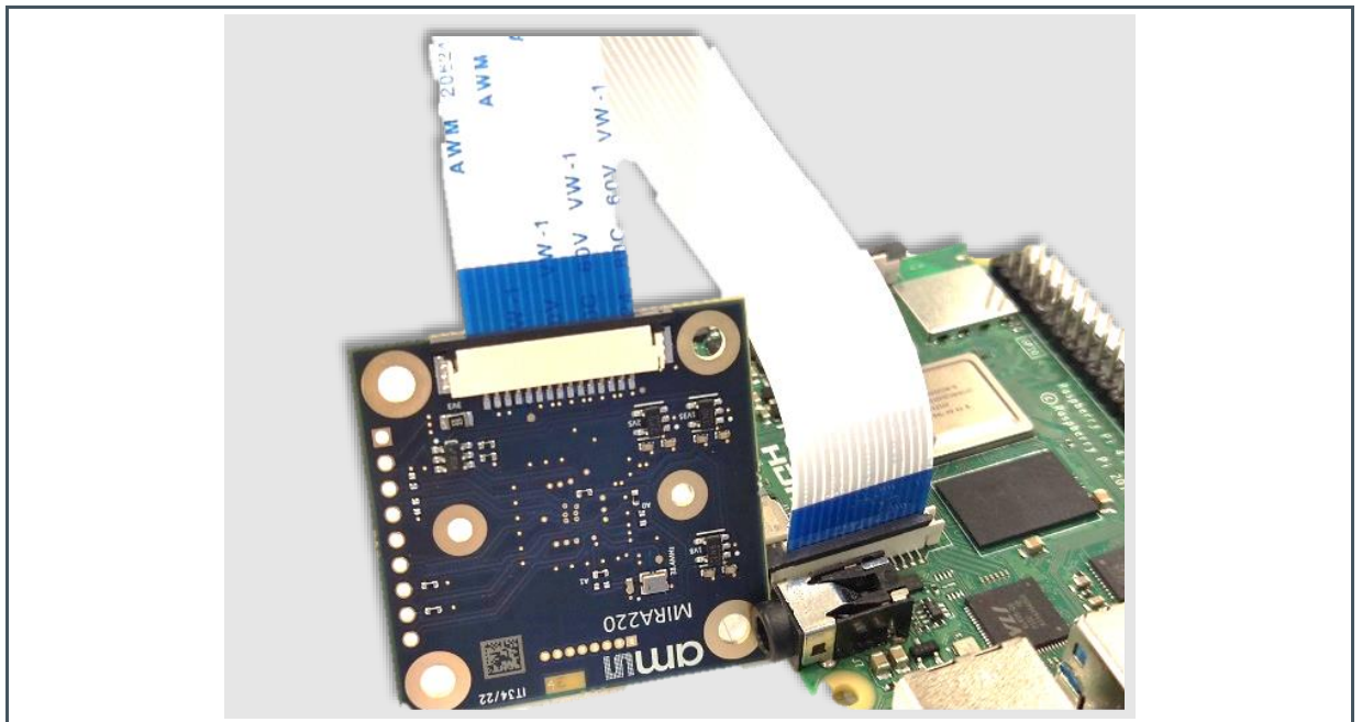
Figure 3: Orientation of the Cable Connection for all Mira220/Mira050 Reference Designs
