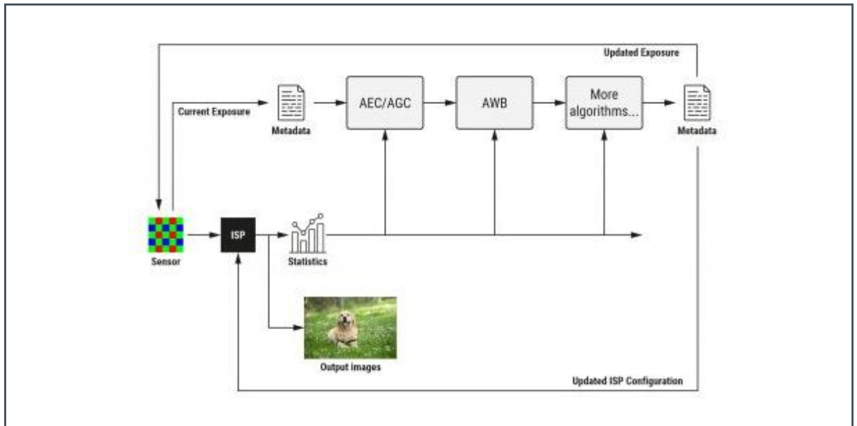
Figure 6: Control Algorithm
