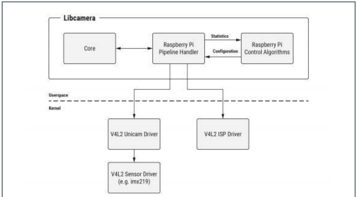
Figure 6: Control Algorithm
